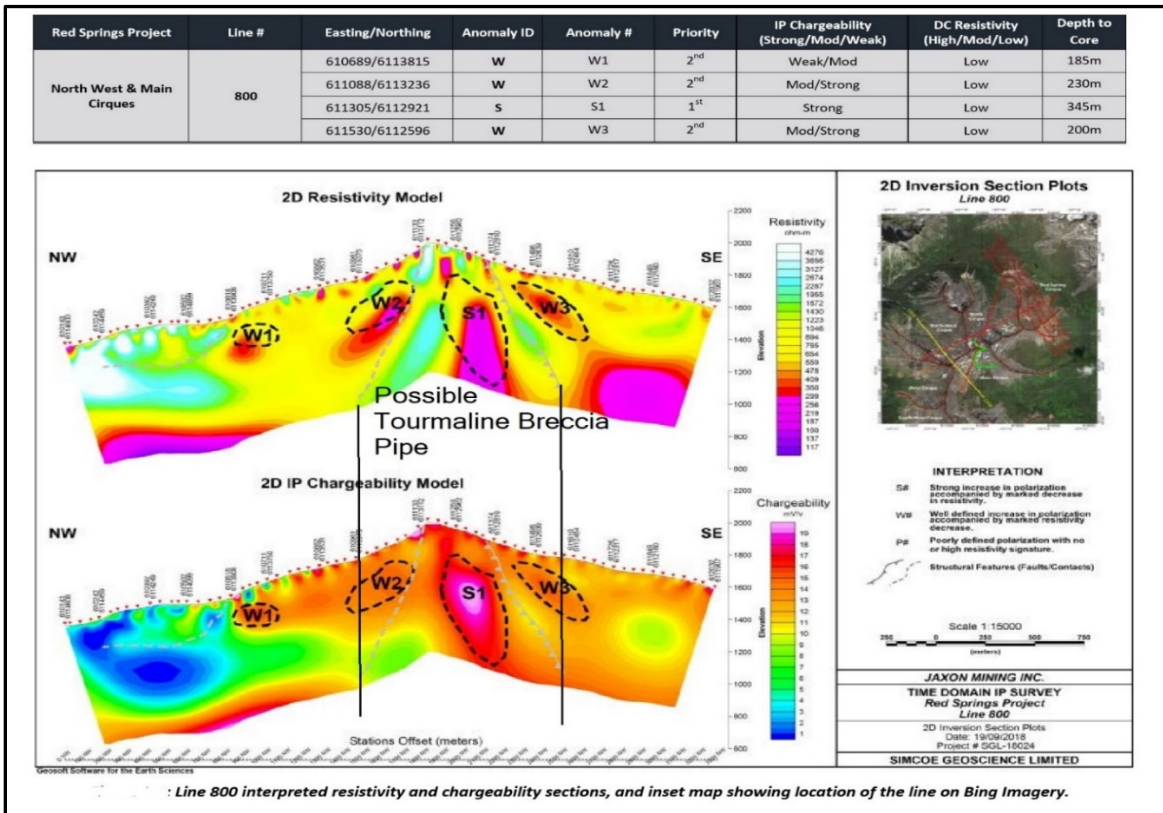
Figure 8 Pipe-like Resistivity and IP Chargeability Anomalies in NW Cirque at Red Springs Project
