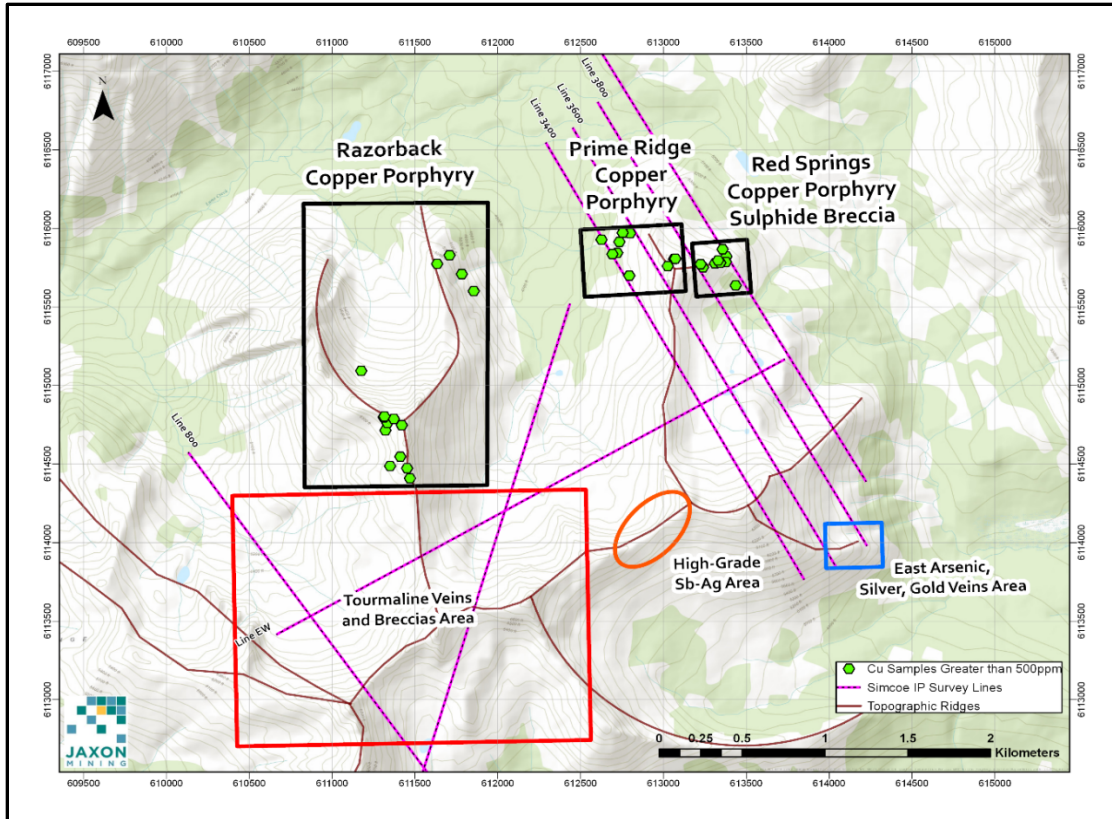
Figure 2, Tourmaline Breccia Mineralization, Two Sulfide Polymetallic Targets and Three Copper Porphyry Targets at Red Springs
