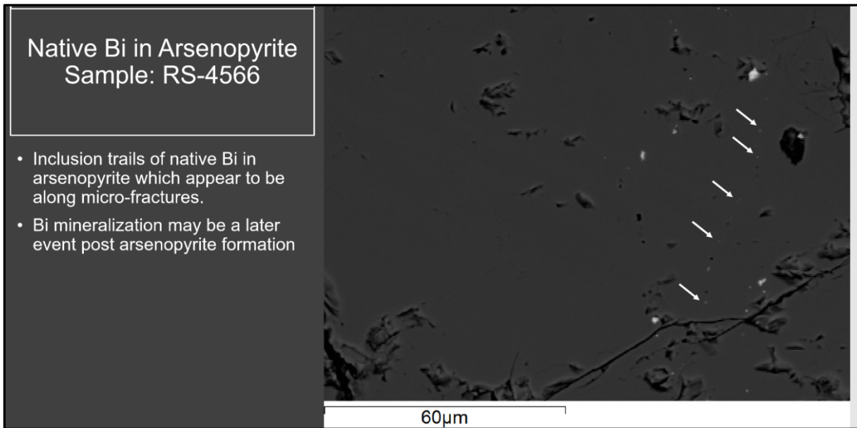
Figure 6, Native Bi in Arsenopyrite From Tourmaline Breccia Sample
