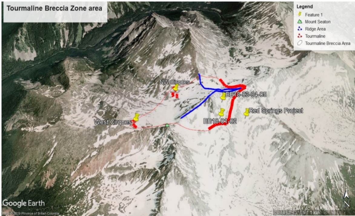
Figure 3, Tourmaline Breccia Zone/Vein Area at Red Springs Project, Red: Tourmaline Breccia, Blue: Ridge Top, BB18-01-05, Drill Pads
