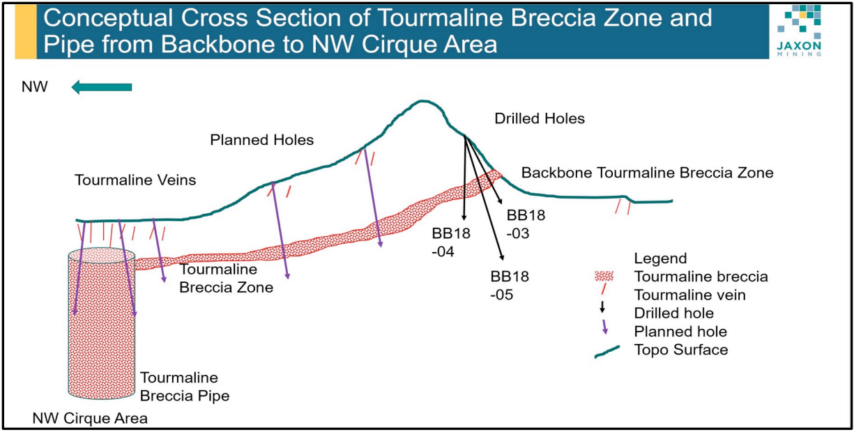
Figure 7, Conceptual Cross Section of Tourmaline Breccia Zone and Pipe from Backbone to NW Cirque Area at Red Springs Project
