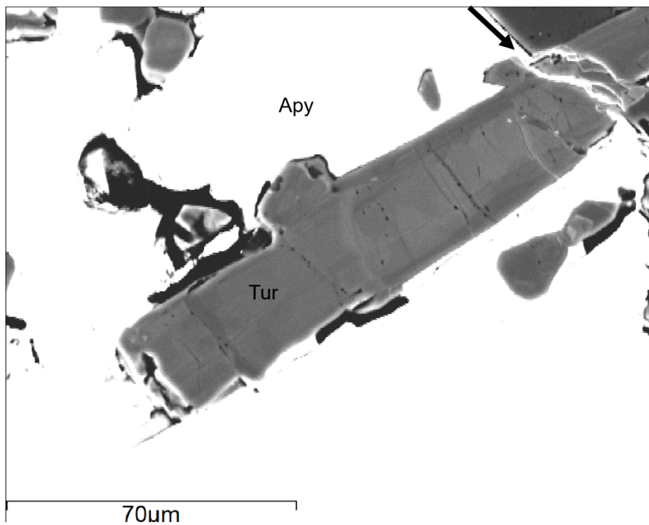
Figure 5, Tourmaline Features and Cross-cut by Arsenopyrite
