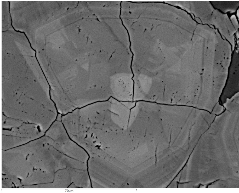
Figure 4, Chaotic Zonation from Tourmaline Breccia at Red Springs
