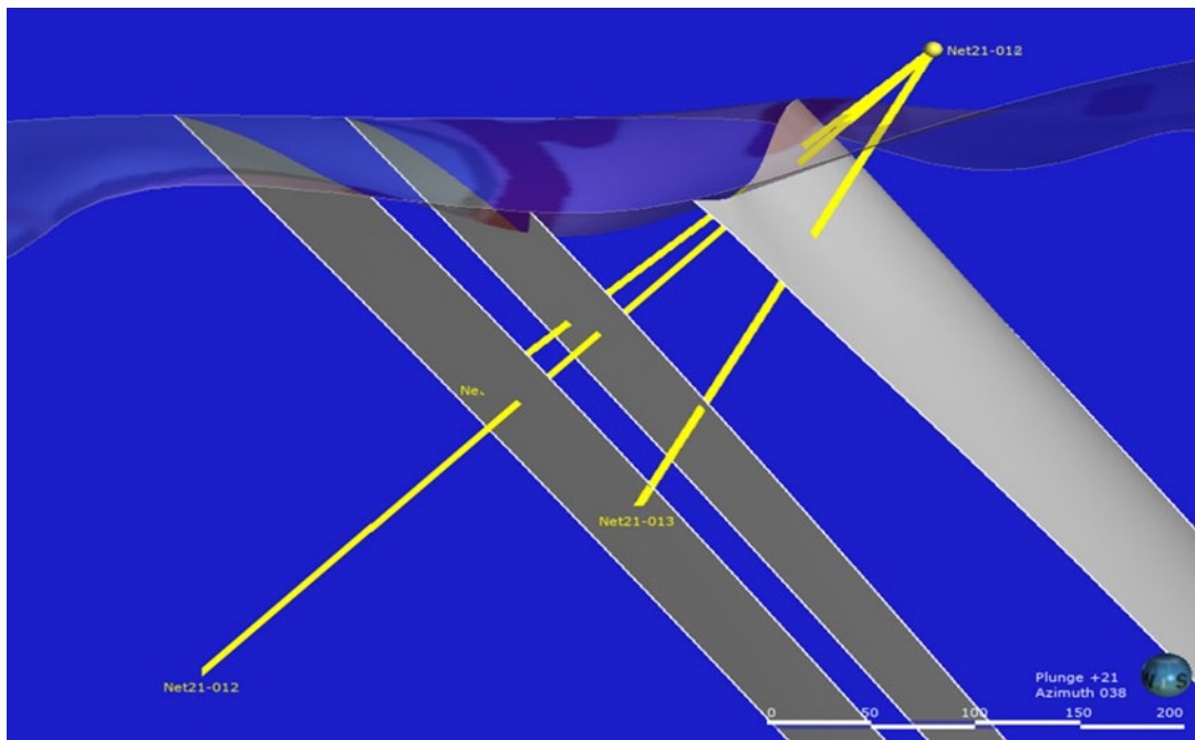
Figure 5. Three angled diamond drill holes will test multiple high-grade Mo-W and Ag-Au-Cu quartz veins at Daisy North Contact Zone to a depth of 50 to 300 metres from surface at pad 5
