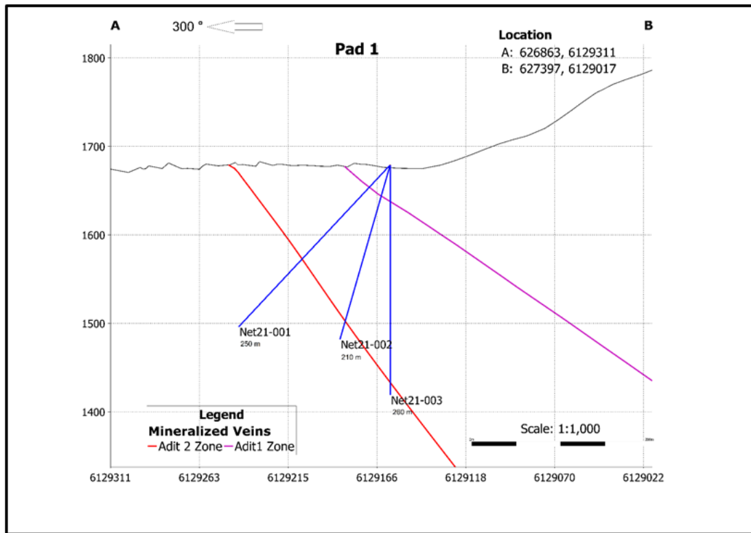
Figure 3. Three diamond drill holes will test Daisy South Adit Zone to a depth of 50 to 250 metres from surface at pad 1
