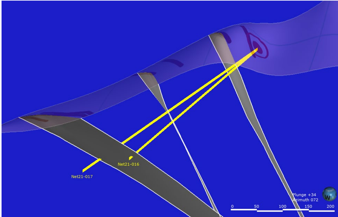
Figure 6. Two angled diamond drill holes will test multiple high-grade Ag-Au-Cu-Mo quartz veins at Daisy Central Zone to a depth of 50 to 300 metres from surface at pad 6
