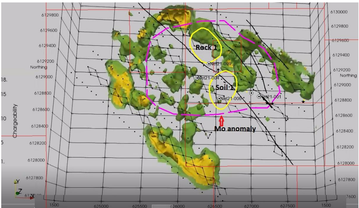
Figure 2. 3D projection of IP chargeability anomalies integrated with the interpreted deep porphyry deposit target areas (yellow line) identified by geochemical footprint 3D modelling within (+50 ppm) Mo in soil anomaly (pink line), and northwest trending deep fault (black line across Mo anomaly)
