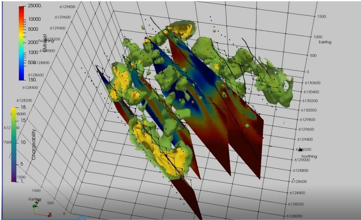
Figure 3. Magnetotelluric and IP survey showing a deep strong and large conductive anomaly (the porphyry system target) ~1,000 m at depth, at central north area surrounded by annular IP chargeability nearer to surface.
