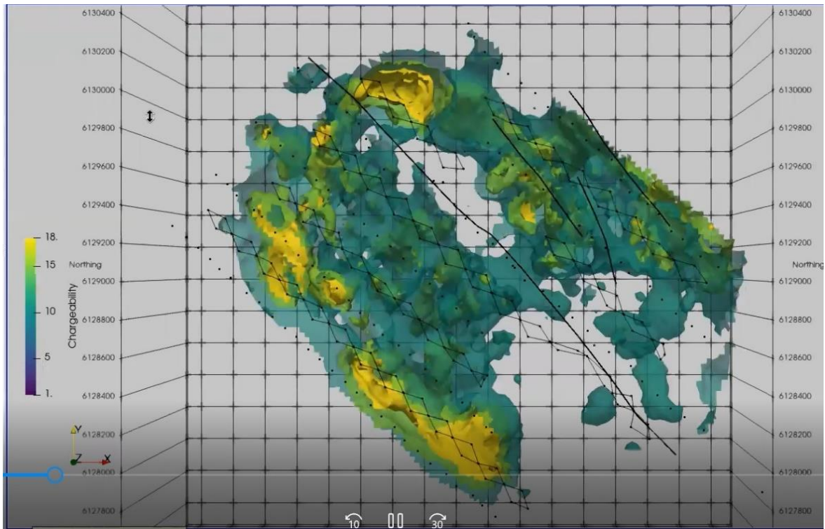
Figure 1. Annular IP chargeability anomaly at Netalzul Mt
