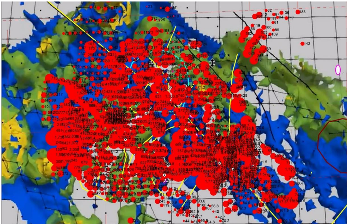
Figure 5. IP chargeability anomaly and Cu-in-soil (+500 ppm) anomaly.
