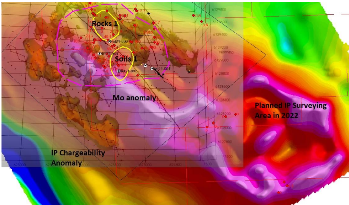
Figure 6. IP chargeability anomaly open to the southeast where IP surveying is planned for 2022.
